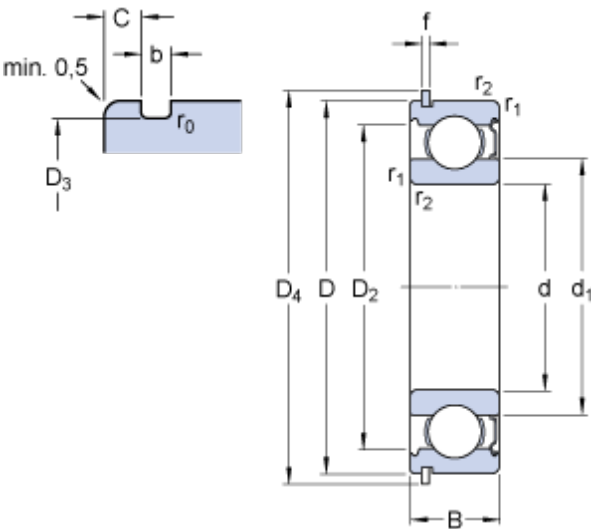
Bearing No. 6201-ZNR
