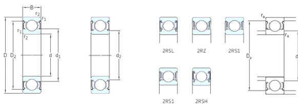
Bearing No. 6201-RSL
