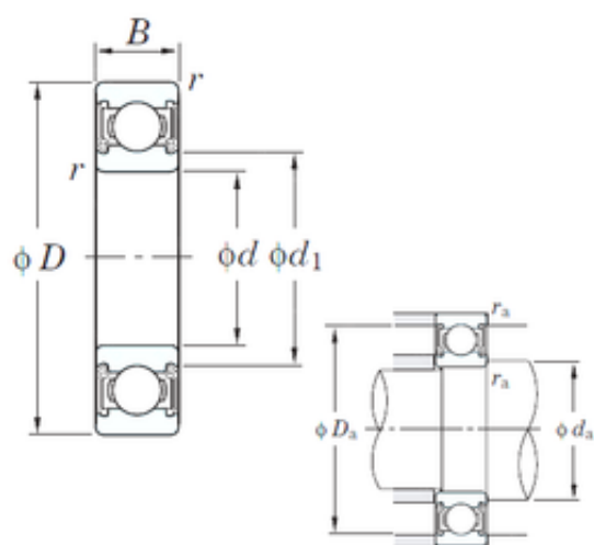
Bearing No. 6201 2RD C3
