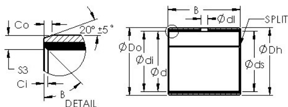
Bearing No. AST11 5540
