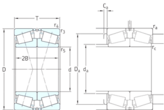
Bearing No. 33018/QDFC150
