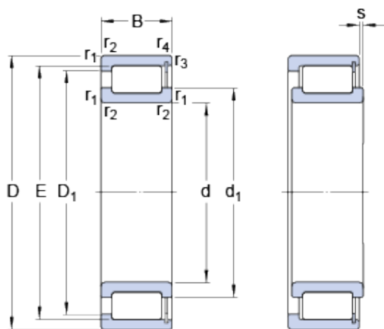
Bearing No. NCF 28/600 V/HB1
