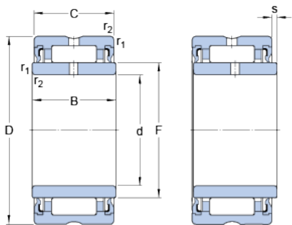
Bearing No. NA 4908.2RS
