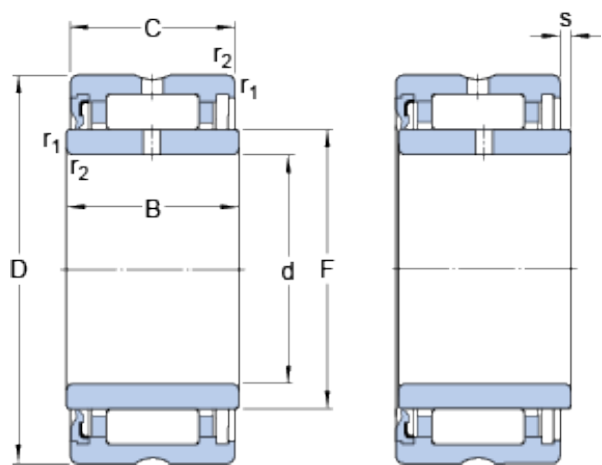
Bearing No. NA 4908 RS
