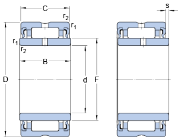
Bearing No. NA 4903.2RS
