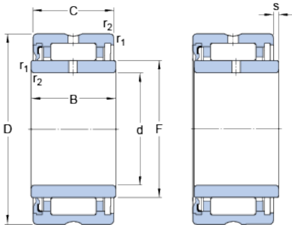
Bearing No. NA 4900 RS
