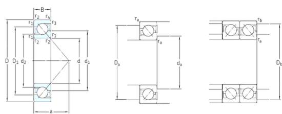
Bearing No. 7030BGM
