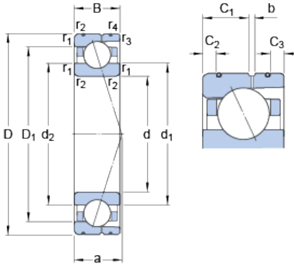
Bearing No. 7030 CD/P4AL
