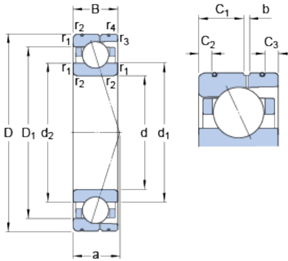
Bearing No. 7030 ACD/P4AL
