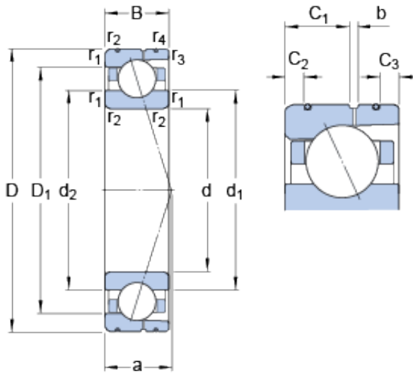
Bearing No. 7030 ACD/HCP4AL
