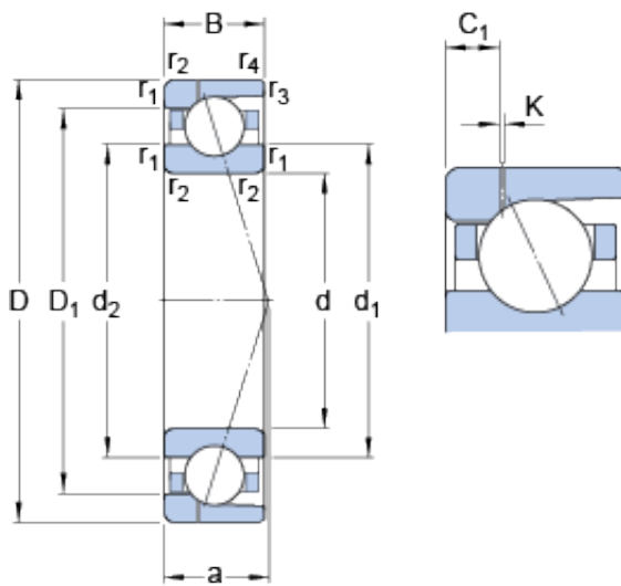
Bearing No. 7030 ACD/HCP4AH1
