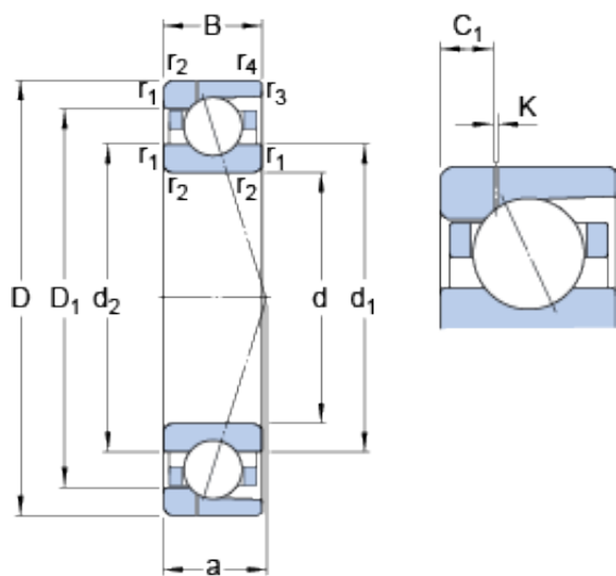
Bearing No. 7028 ACD/P4AH1
