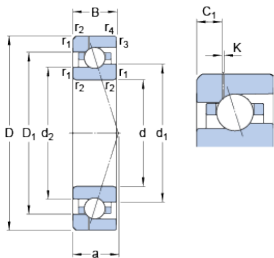
Bearing No. 7024 CE/P4AH1
