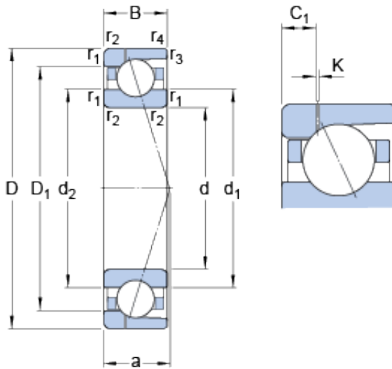
Bearing No. 7021 ACD/HCP4AH1
