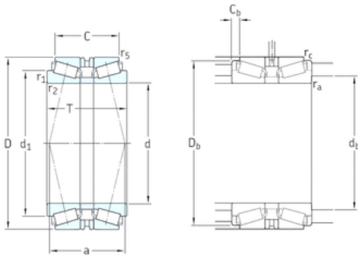
Bearing No. 32220T140J2/DB11
