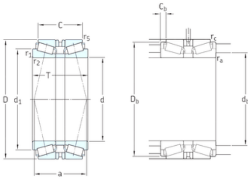
Bearing No. 32220T108J2/DB
