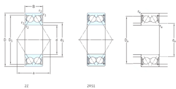
Bearing No. E2.3205A-2Z
