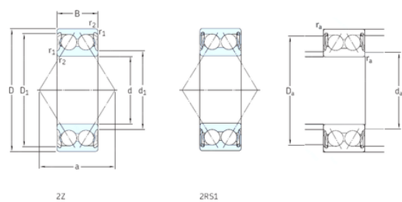
Bearing No. E2.3308A-2Z
