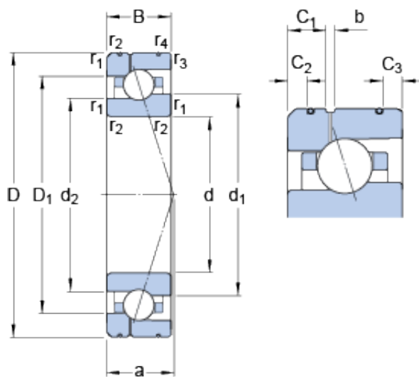
Bearing No. 7017 CE/P4AL1
