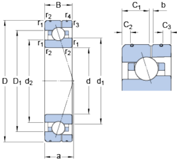
Bearing No. 7017 ACE/HCP4AL
