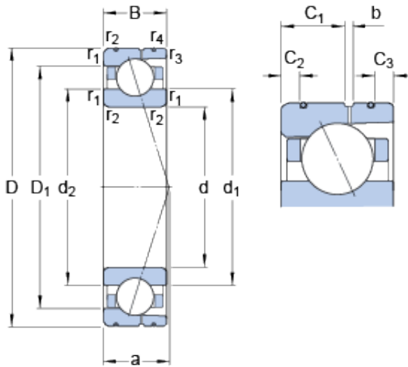
Bearing No. 7017 ACD/P4AL
