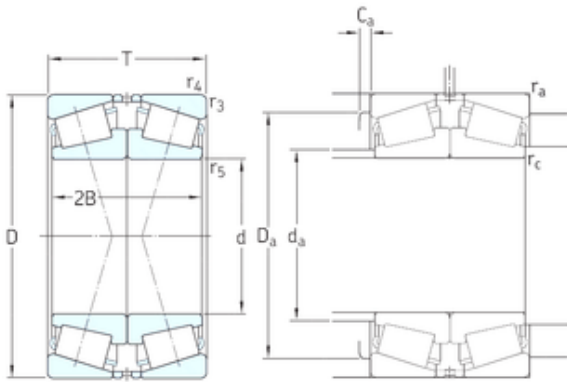
Bearing No. 32044X/DF
