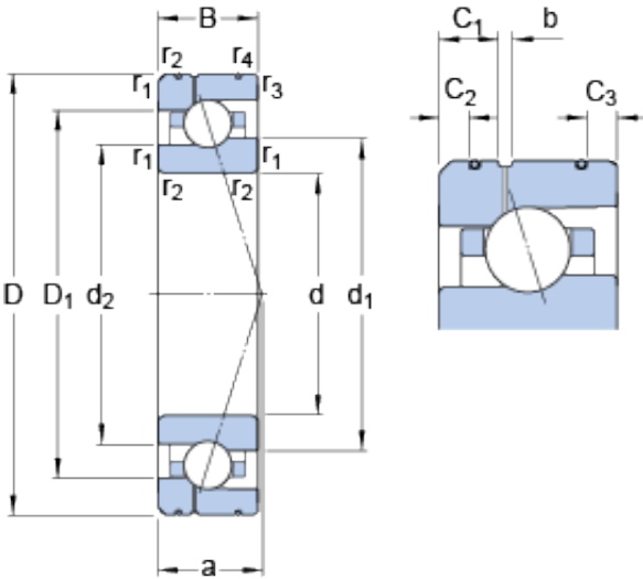
Bearing No. 7016 CE/P4AL1
