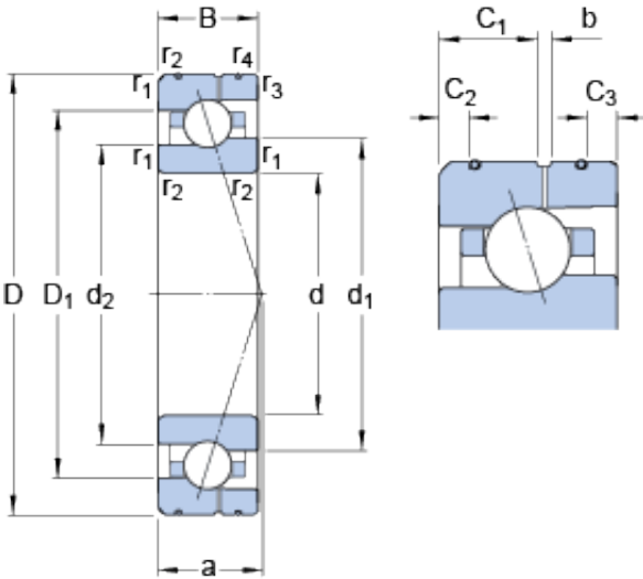
Bearing No. 7016 ACE/P4AL
