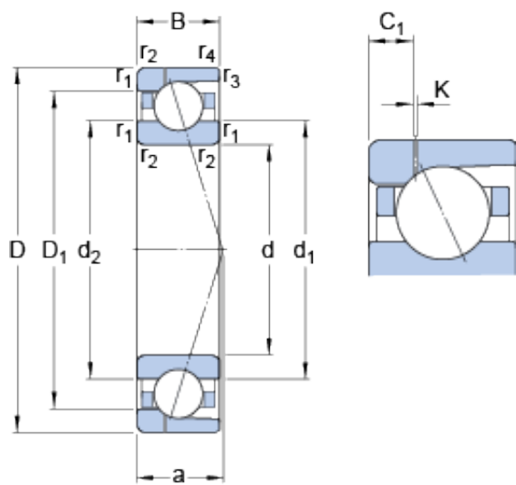
Bearing No. 7016 ACD/P4AH1
