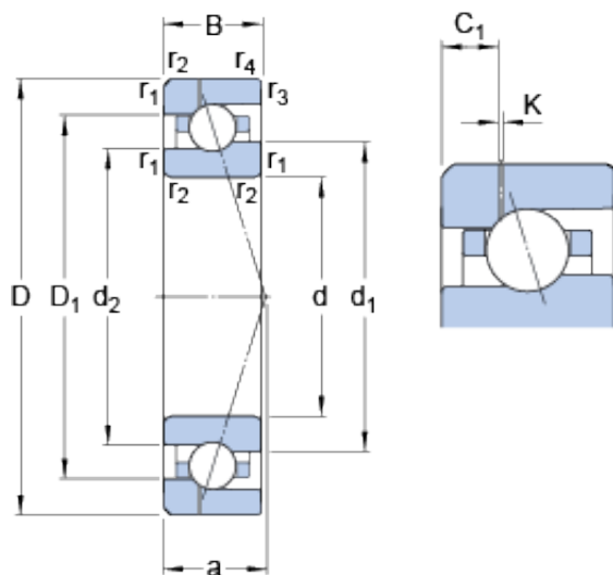
Bearing No. 7015 CE/HCP4AH1
