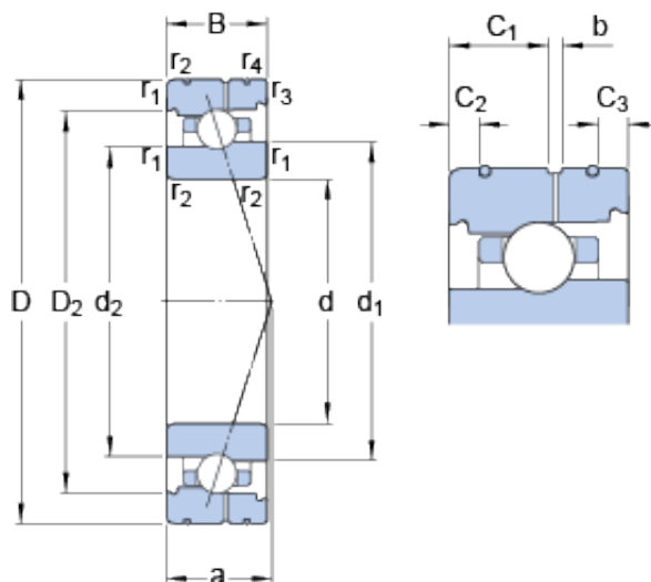
Bearing No. 7015 CB/HCP4AL
