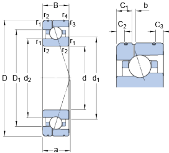
Bearing No. 7015 ACE/P4AL1
