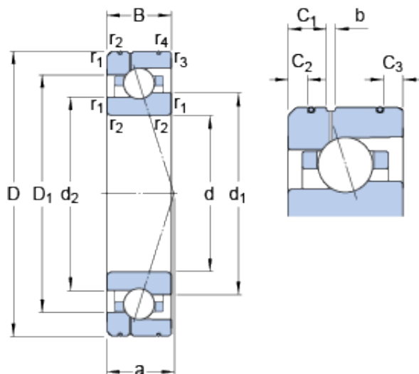
Bearing No. 7015 ACE/HCP4AL1
