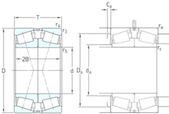
Bearing No. 32022X/QDF
