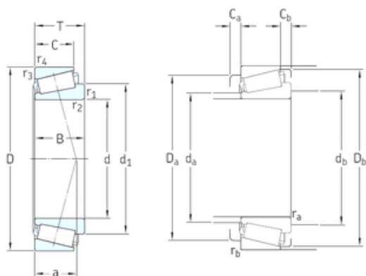
Bearing No. 32013X/Q
