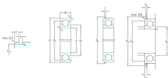
Bearing No. 6021N
