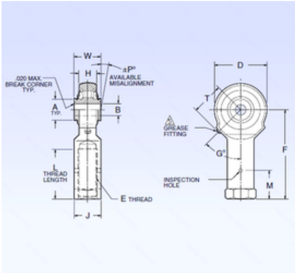
Bearing No. ARR4FFN-1B
