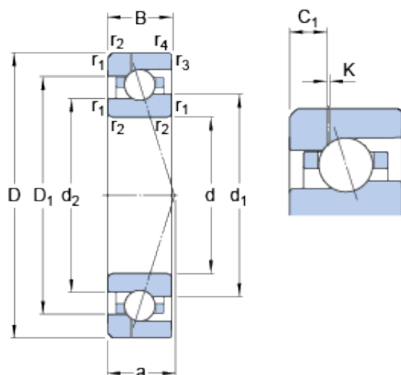
Bearing No. 7011 ACE/P4AH1
