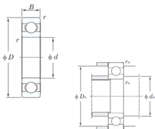
Bearing No. 16008
