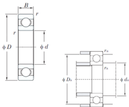
Bearing No. 6017
