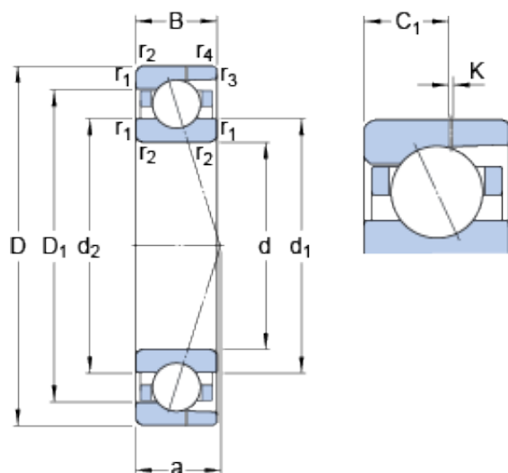
Bearing No. 7007 CD/HCP4AH
