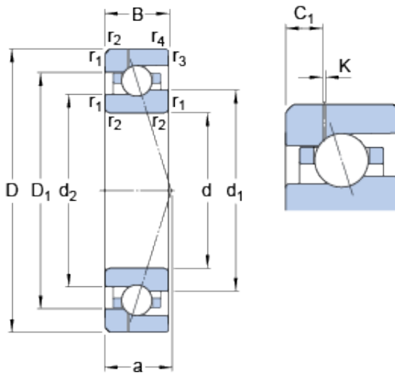
Bearing No. 7007 ACE/P4AH1
