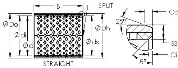
Bearing No. AST090 6030
